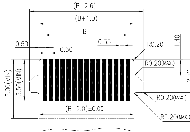
APPLICABLE FPC/FFC
